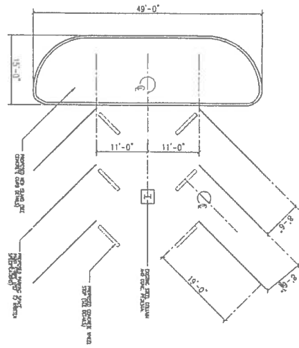
ISLAND NO. 3, WHEEL STOP, AND STRIPING PARTIAL PLAN
