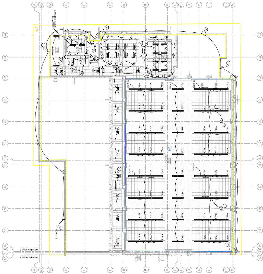
SECOND FLOOR LIGHTING PLAN - SECTOR B
